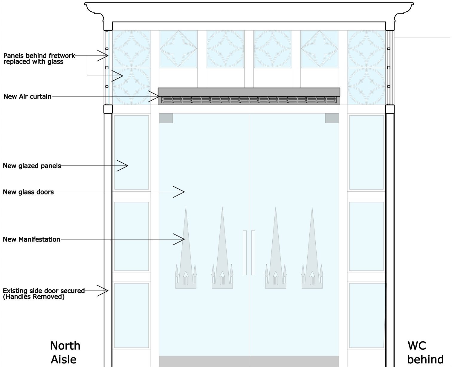
Section DD - Lobby cross section looking South
