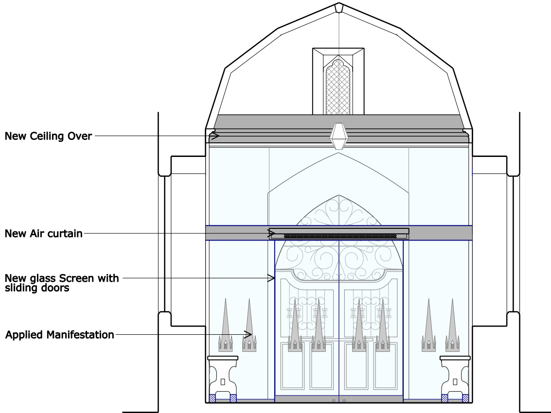
Section BB - Porch Cross section looking North
