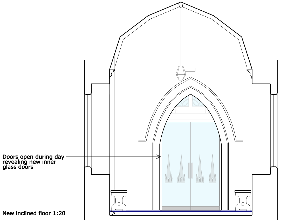
Section AA - Porch cross section looking South
